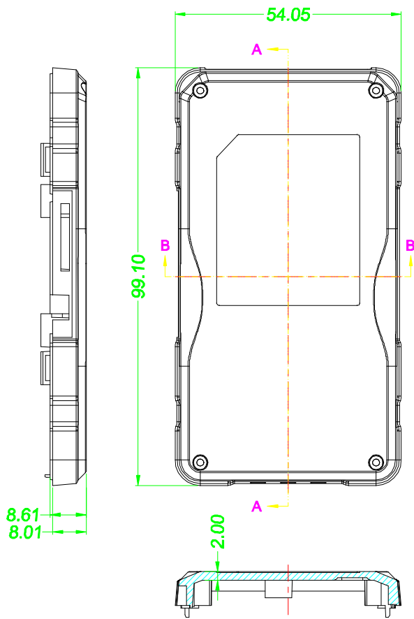
SECTION B-B
